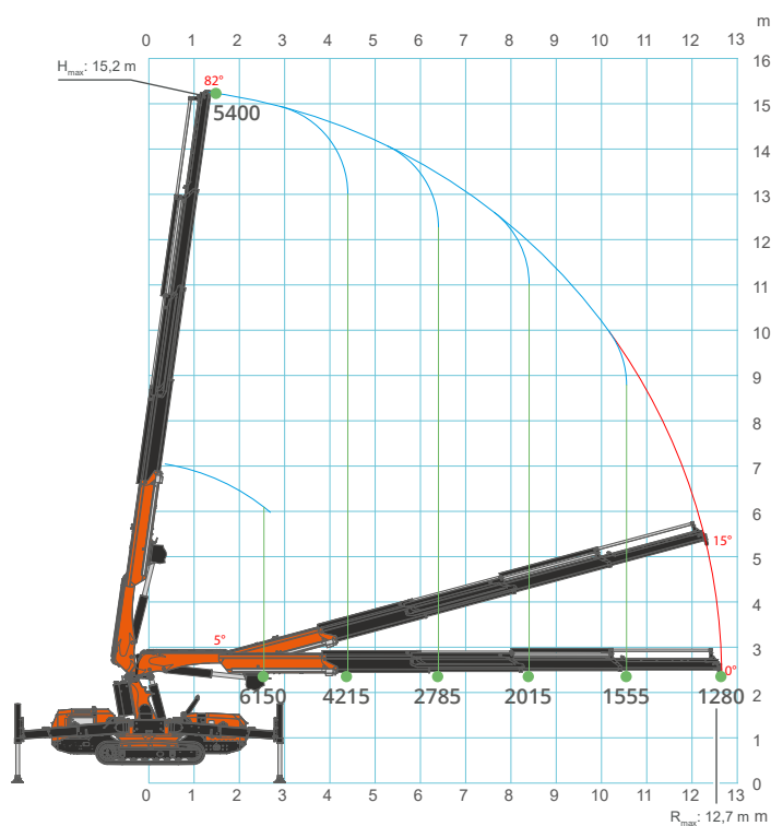
Main Boom
