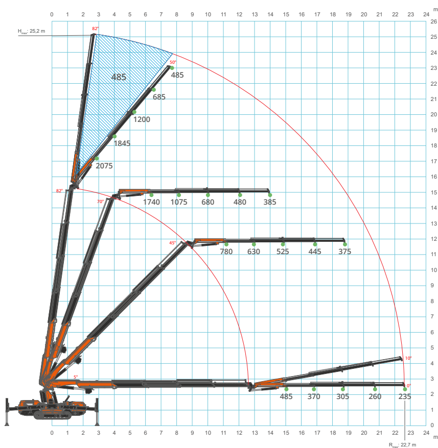
Hydraulic Jib
