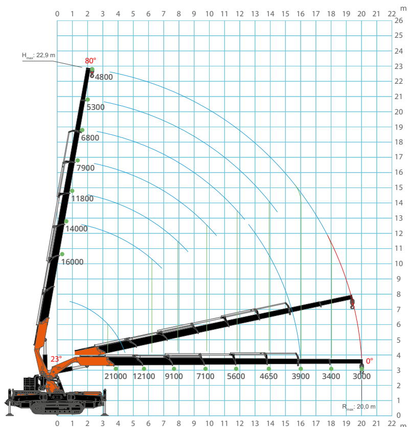
Main Boom
