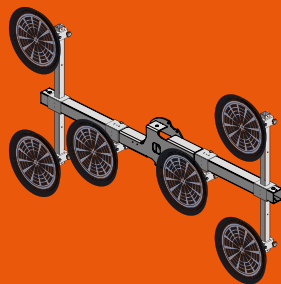
Ø400 – 6 ventouses
