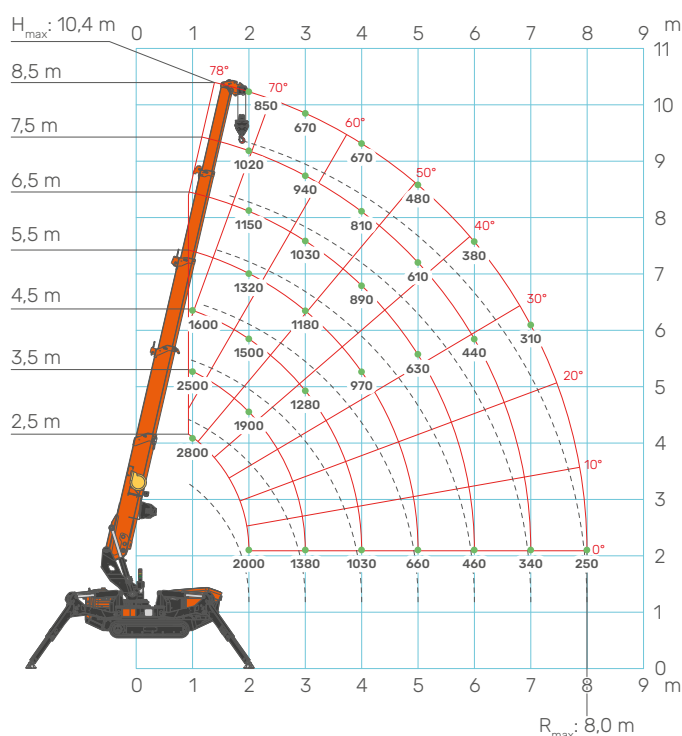
Brazo Principal
