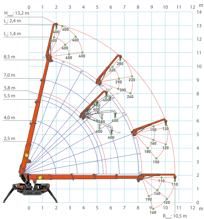
Mechanical Jib
