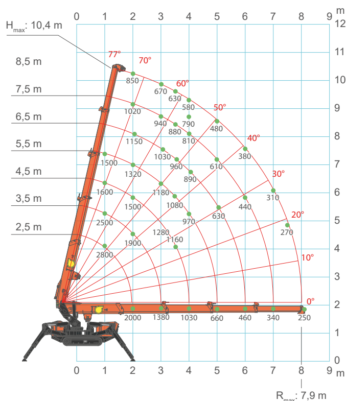
Main Boom
