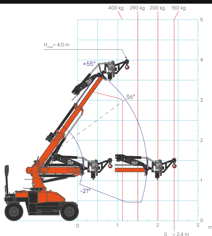
Manipulator Hook Load Chart
